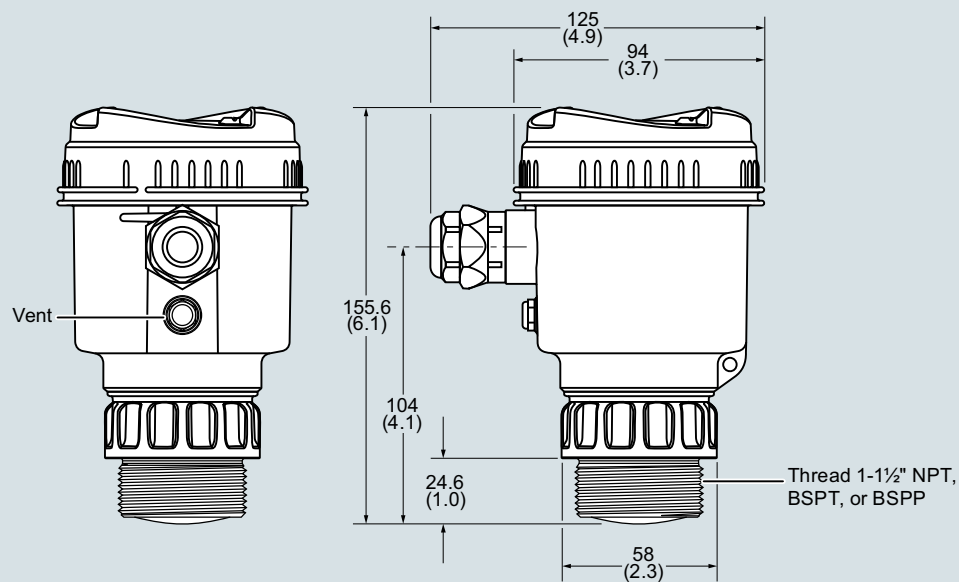
SITRANS LR150, dimensions in mm (inch)
