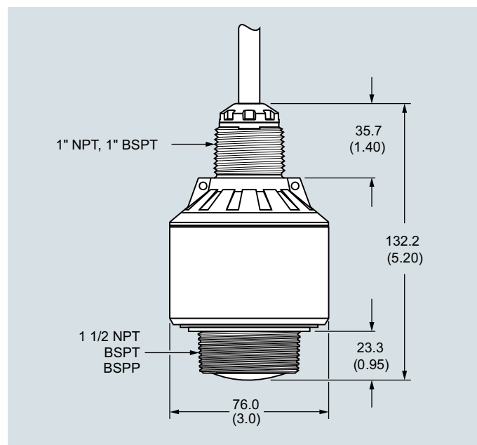
SITRANS LR110, dimensions in mm (inch)
