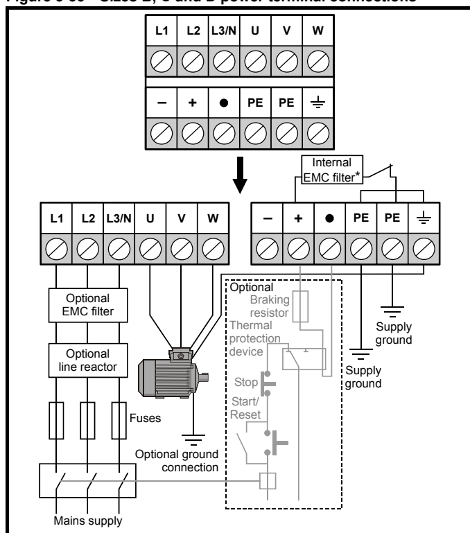
Figure 5-36 Sizes B, C and D power terminal connections
