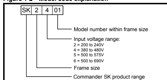
Figure 1-2 Model code explanation
