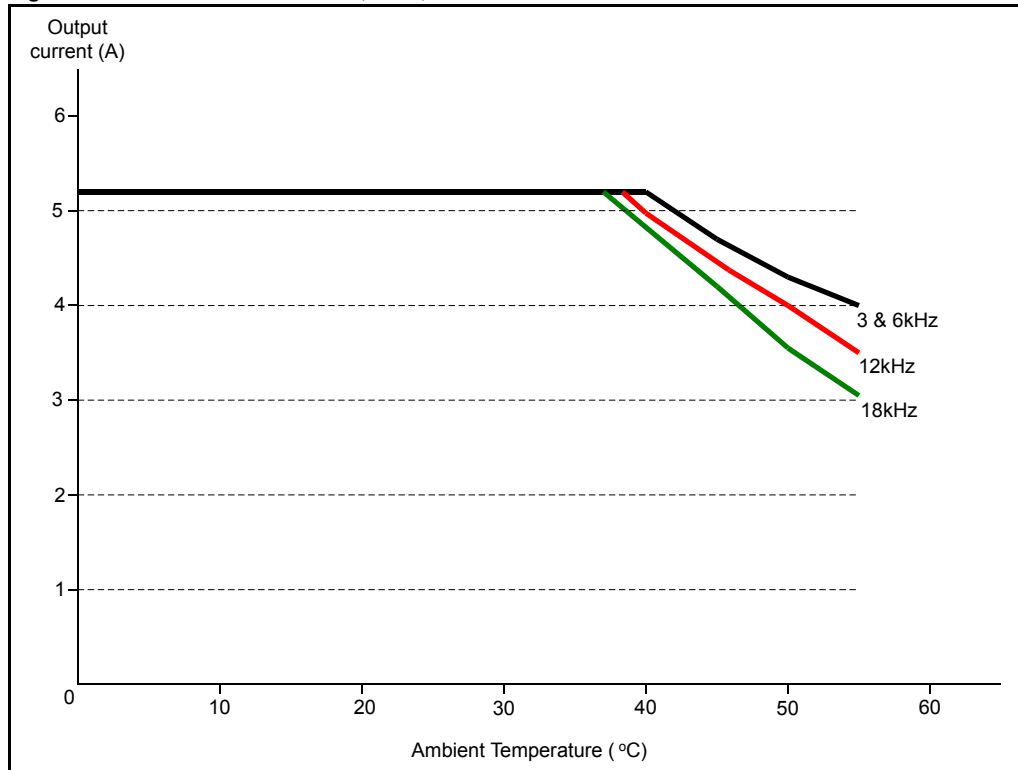
Figure 2-5 Commander SK Size B, 200V, 1.1kW
